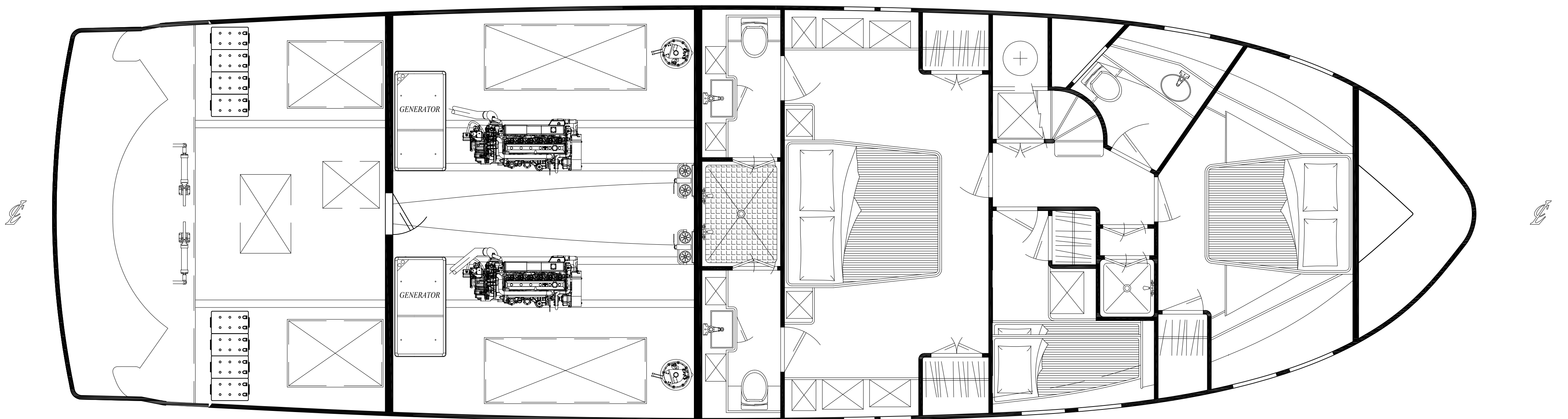
NW-63 GALLEY UP - THREE STATEROOM - VERSION "B"
