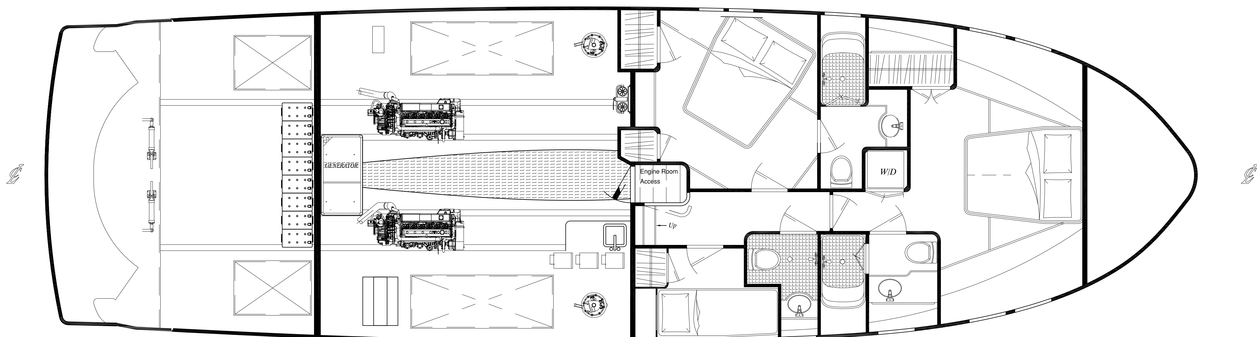
NW-63 GALLEY DOWN - THREE STATEROOM - VERSION "D"
