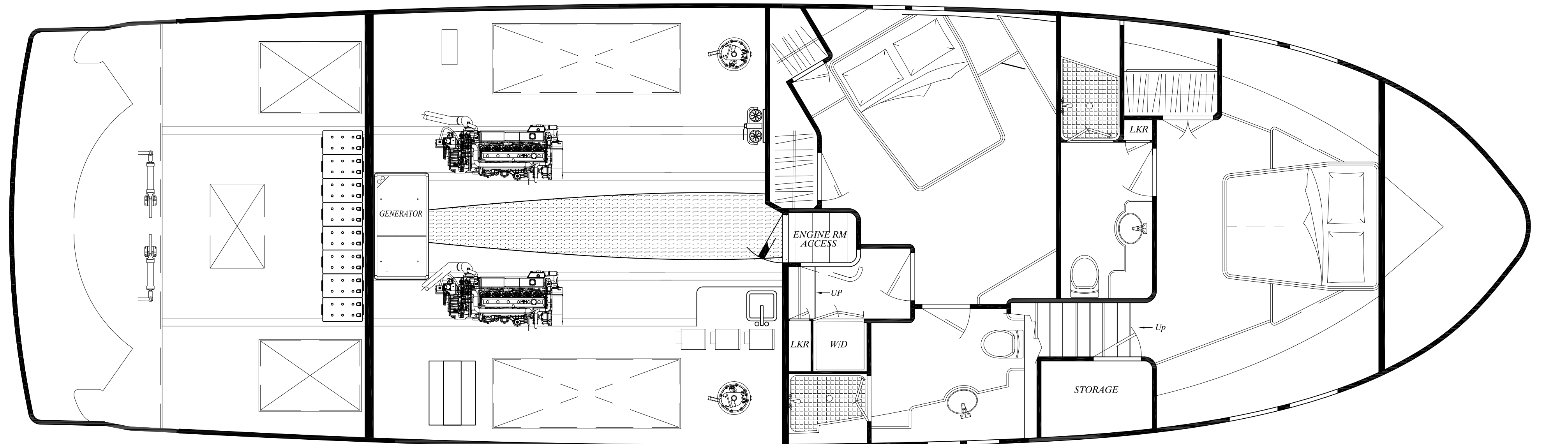
NW-63 GALLEY DOWN - TWO STATEROOM - VERSION "C"
