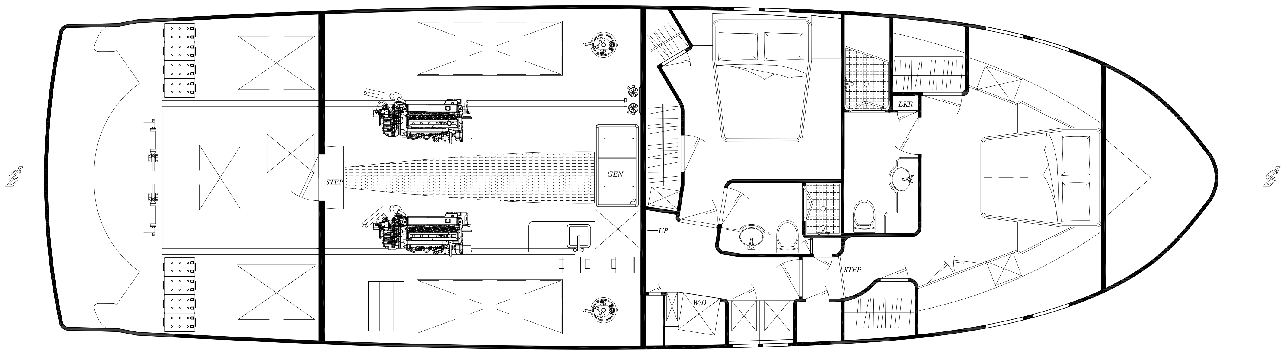
NW-63 GALLEYDOWN - TWO STATEROOM - VERSION "A"
